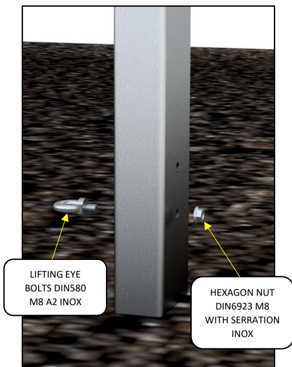
DETAIL L
