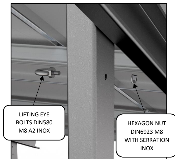
DETAIL J
