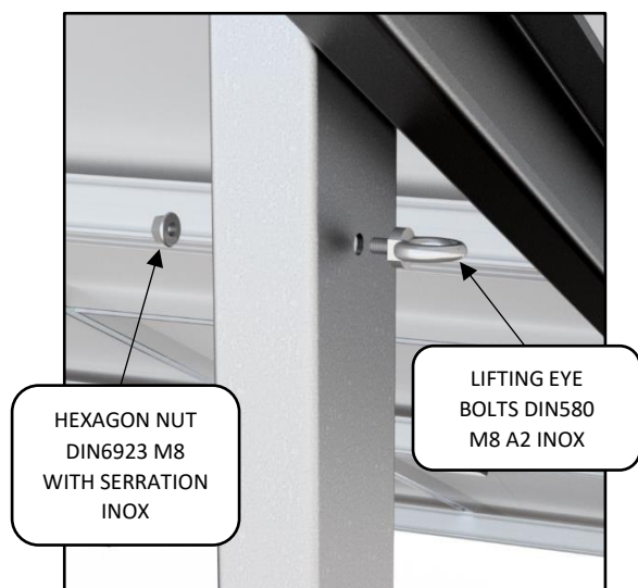
DETAIL I
