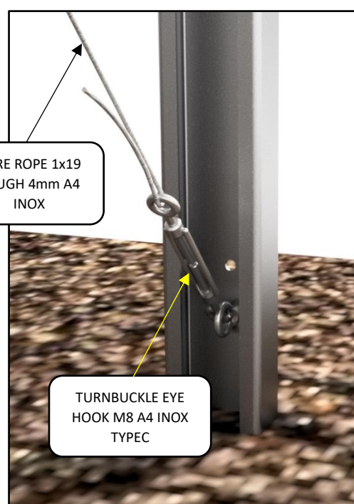
DETAIL N
