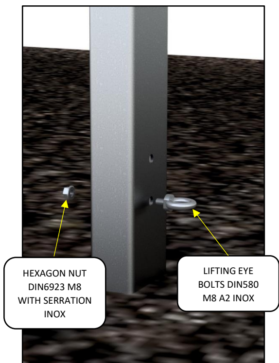
DETAIL K
