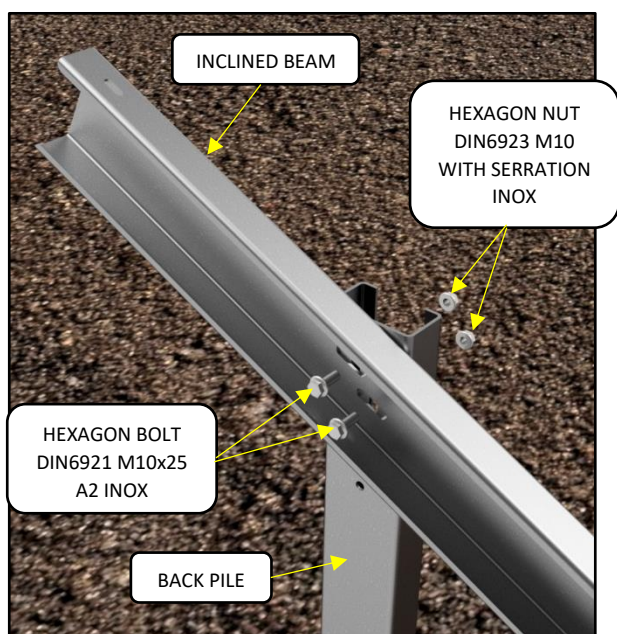
DETAIL B
