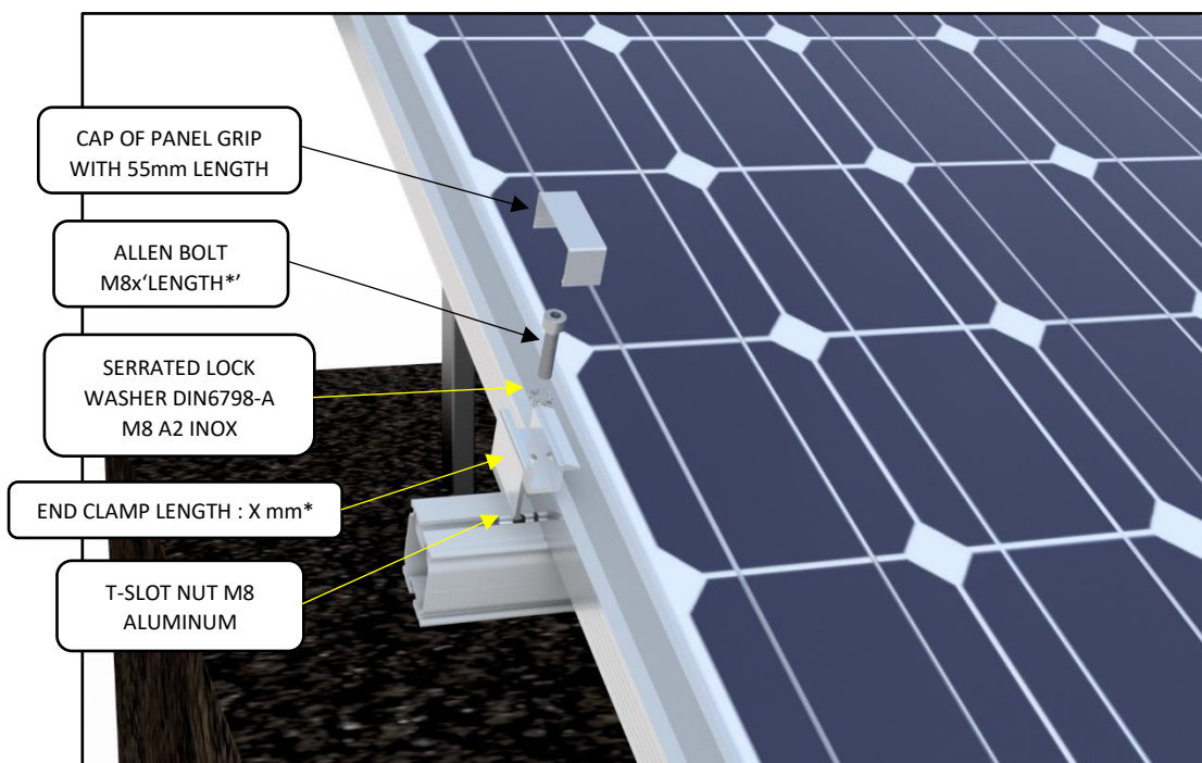
DETAIL F
