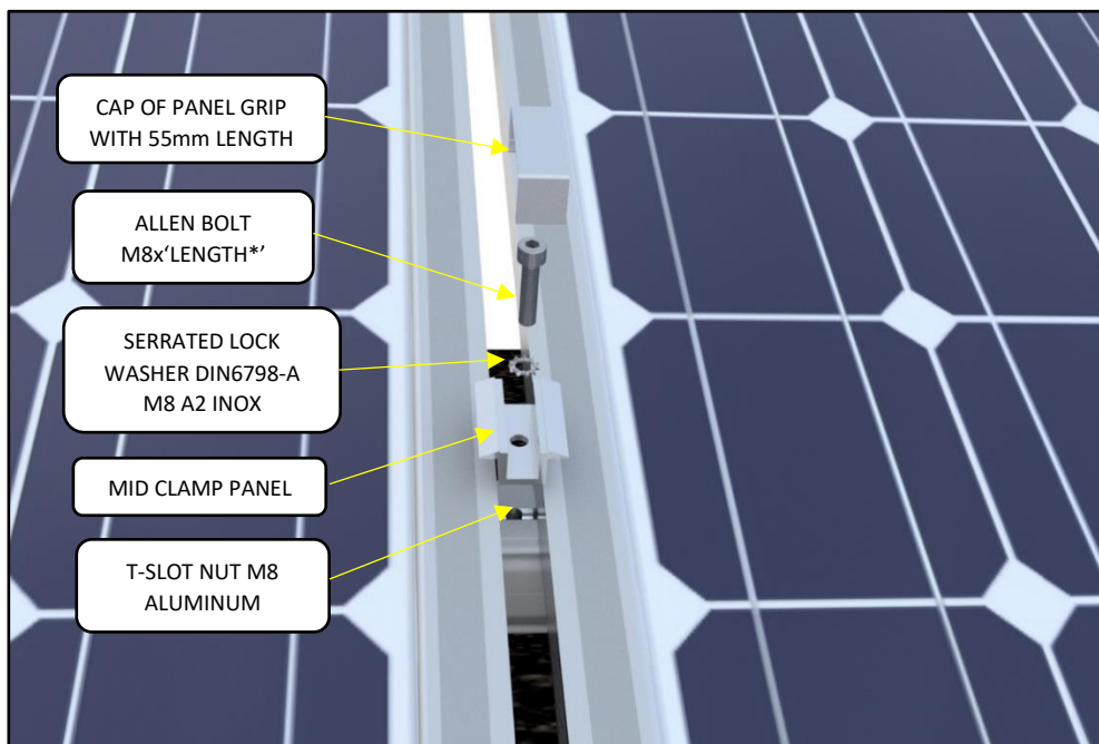
DETAIL G
