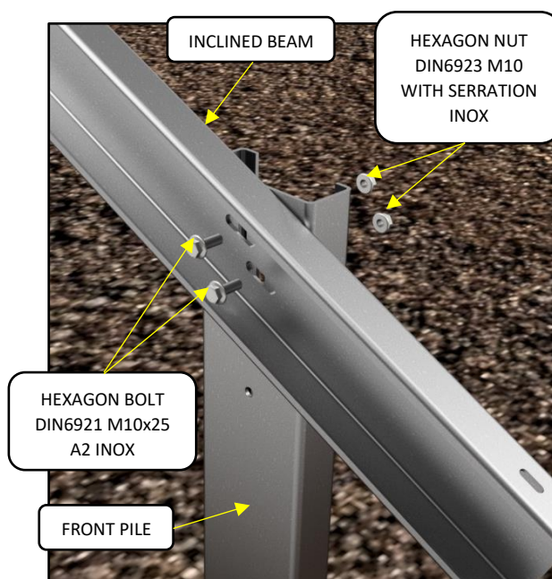
DETAIL C
