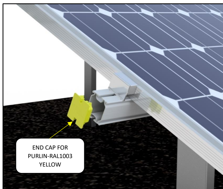
DETAIL H
