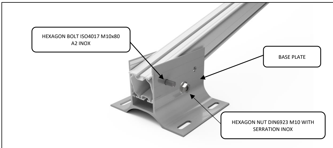
DETAIL C
