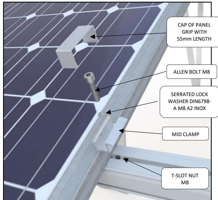
DETAIL G
