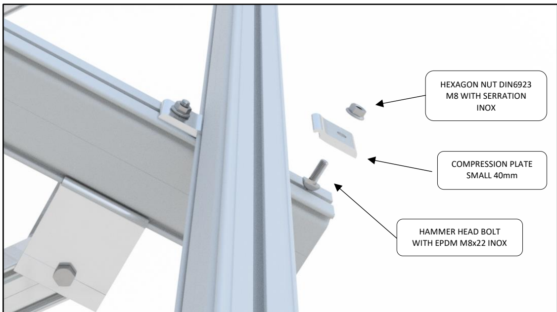
DETAIL D
