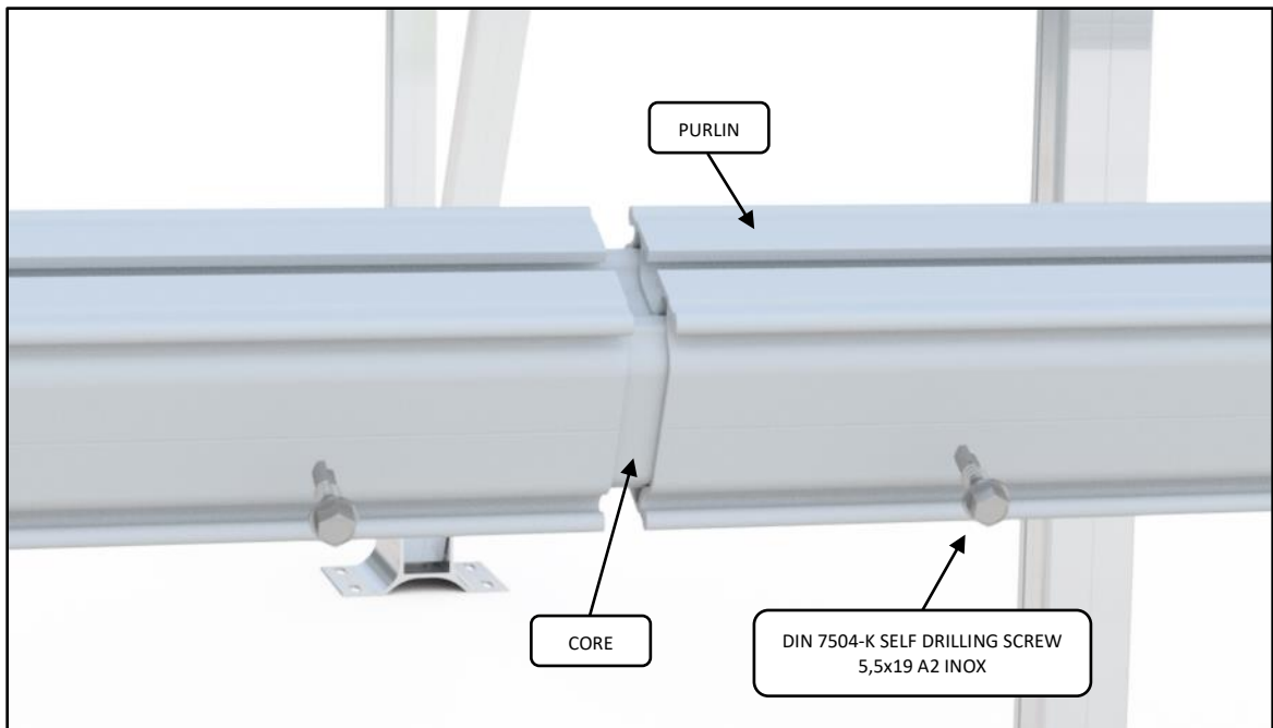
DETAIL E
